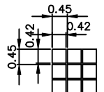
A DETAIL
