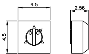
B DETAIL
