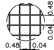
A DETAIL 1:10
