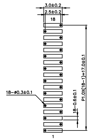
A (DETAIL of INTERFACE TERMINAL)
