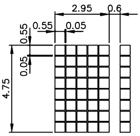
DOT DETAIL
