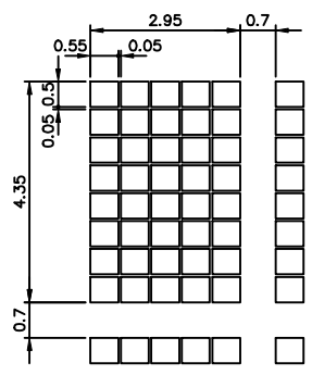
16CX2L A DETAIL
